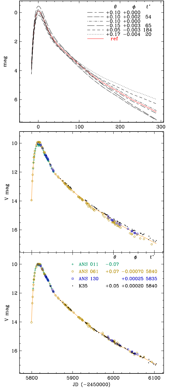
Figure 2: Example of the lightcurve merging method (LMM) described in Sect. 3. Top : These lightcurves are the results of shifting (by \theta ) and stretching (by \phi ) around the pivot points ( t^* ) the ordinates (magnitudes) of the reference lightcurve (plotted in red). Middle : our source V -band observations for SN 2011fe, where different colors and symbols identify different telescopes. Bottom : our merged V -band lightcurve of SN 2011fe after application (by the given quantities) of the LMM shift and pivot stretching method. The orange line (the same in both the middle and bottom panels) is a spline fit to the merged lightcurve \text{mag}(\lambda)_{i,j} (cf. Eq.(3)).
